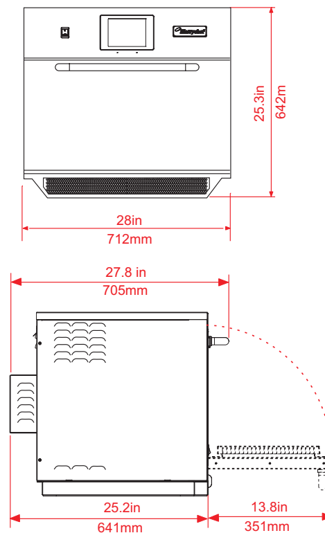
Oven Dimensions
